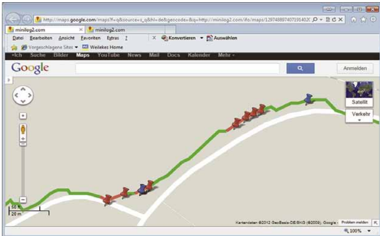
DCVG measurement export to Google® Maps for defect localization
