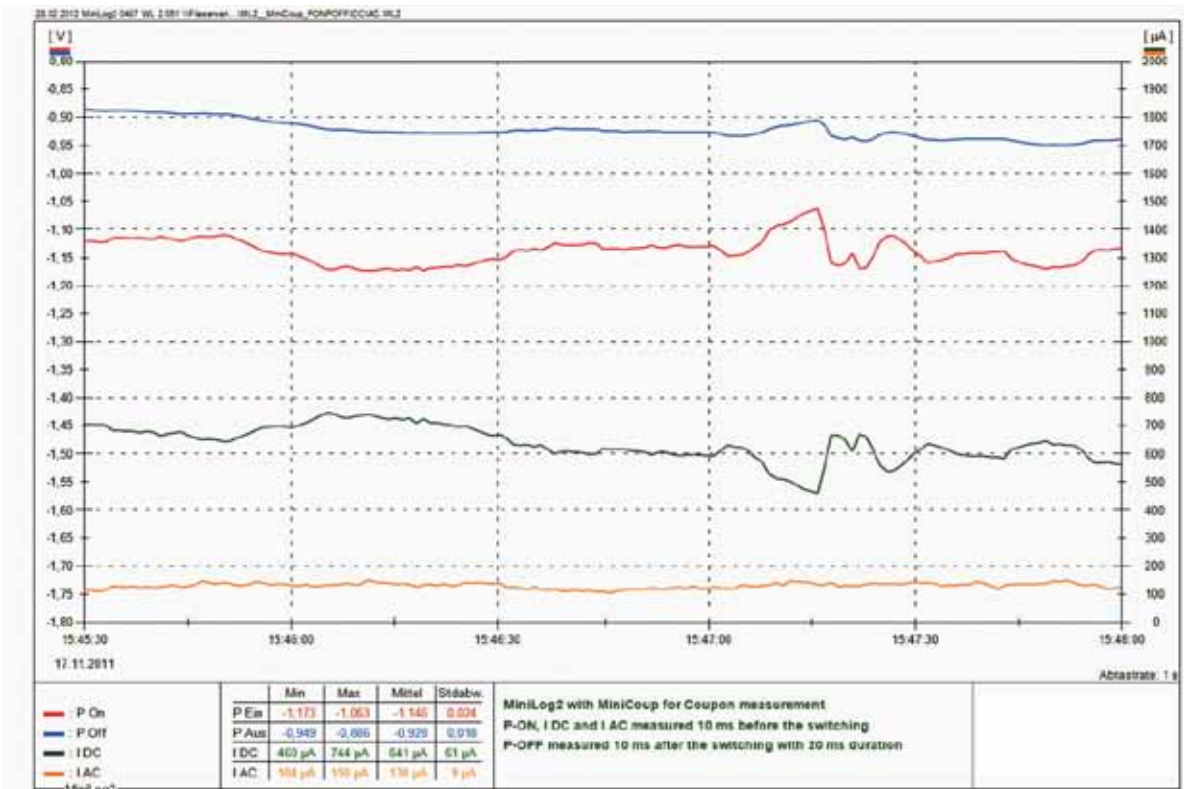
Print: 24 hours coupon measurement with P_{ON} + P_{OFF} + I_{DC} + I_{AC}
