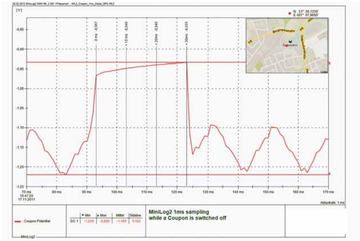
Print: Coupon switching with 1 ms sampling rate
